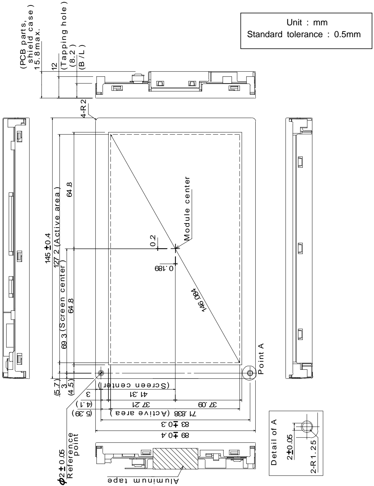
Figure 1. Front View
