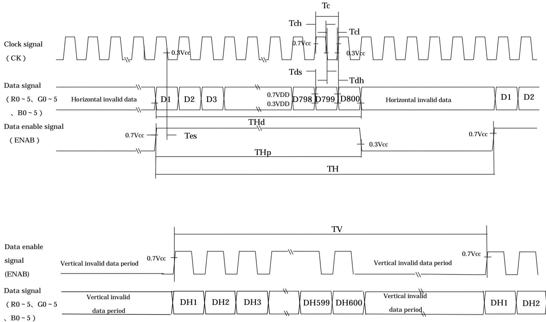
fig1. Input signal timing
