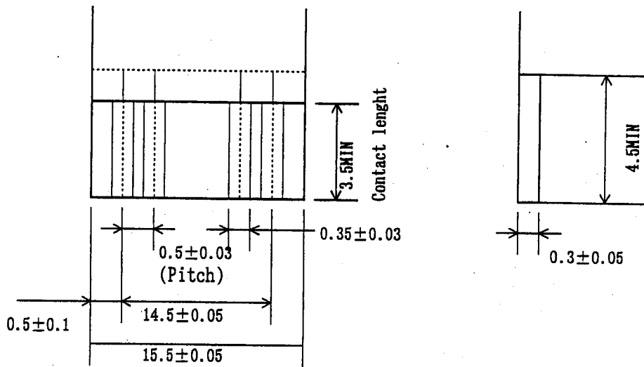
Fig.4 Corresponding FPC dimension
